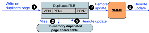
Fig. 13. Workflow of remote update
